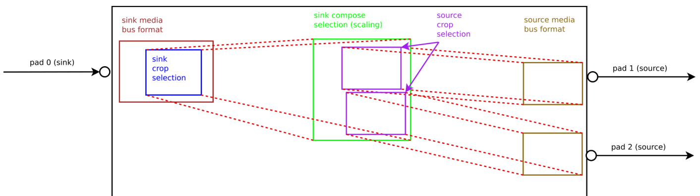
Fig. 1.13: Figure 4.6. Image processing in subdevs: scaling with multiple sources
