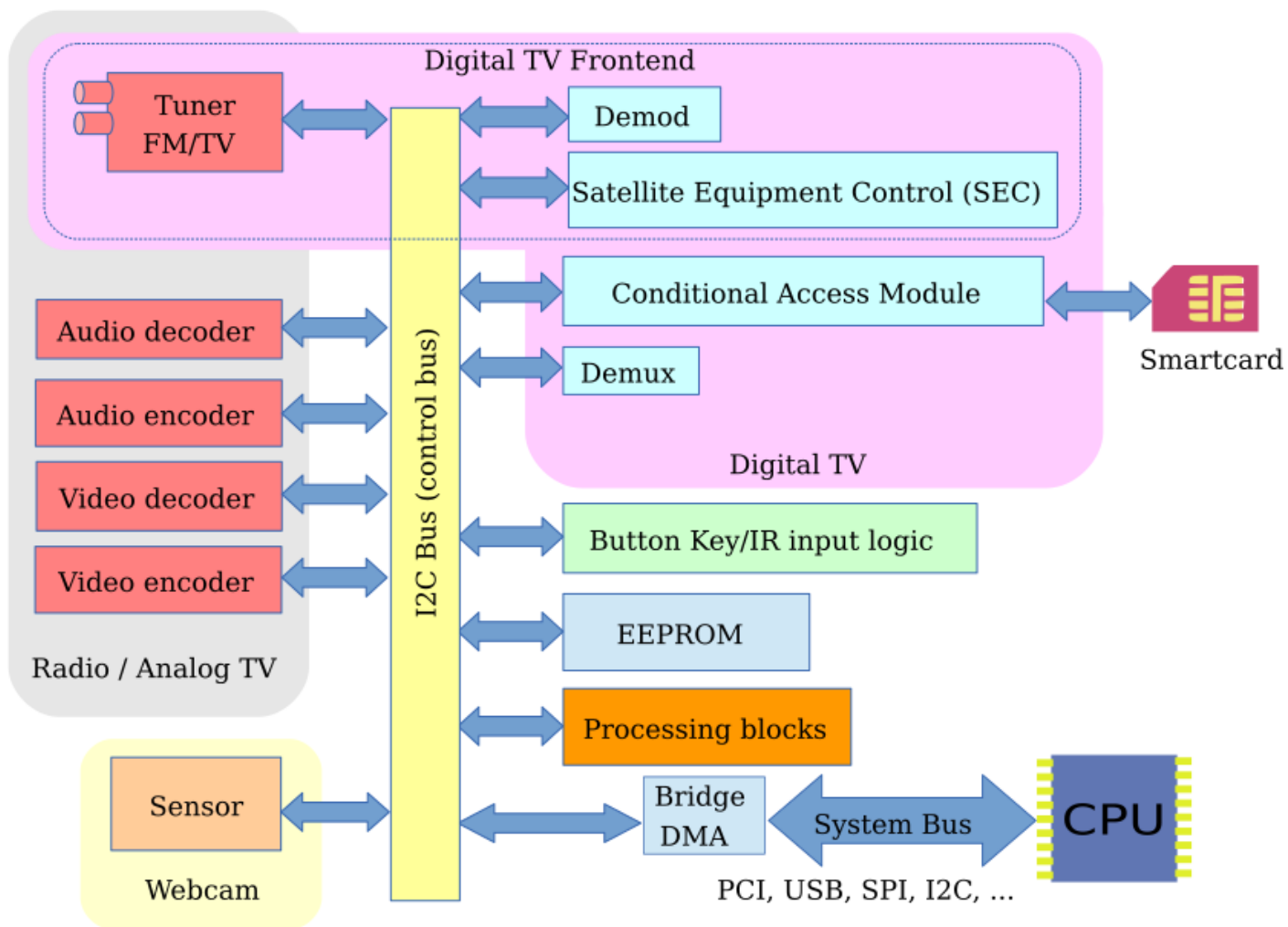
Fig. 1.1: Typical Media Device
