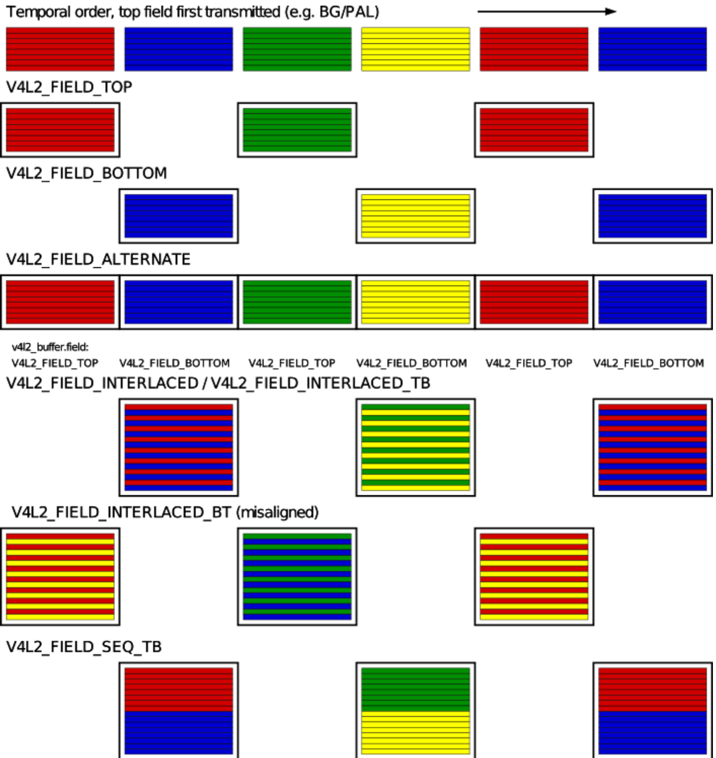
Fig. 1.6: Field Order, Top Field First Transmitted
