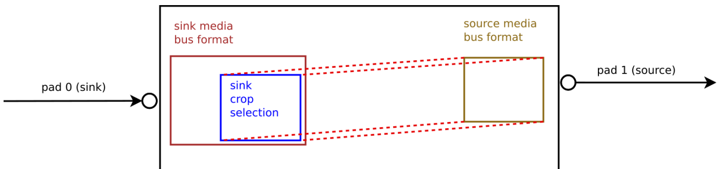
Fig. 1.12: Figure 4.5. Image processing in subdevs: simple crop example
