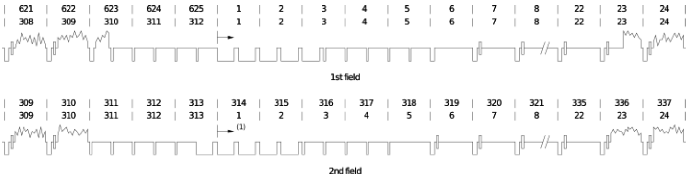
Fig. 1.10: Figure 4.3. ITU-R 625 line numbering
