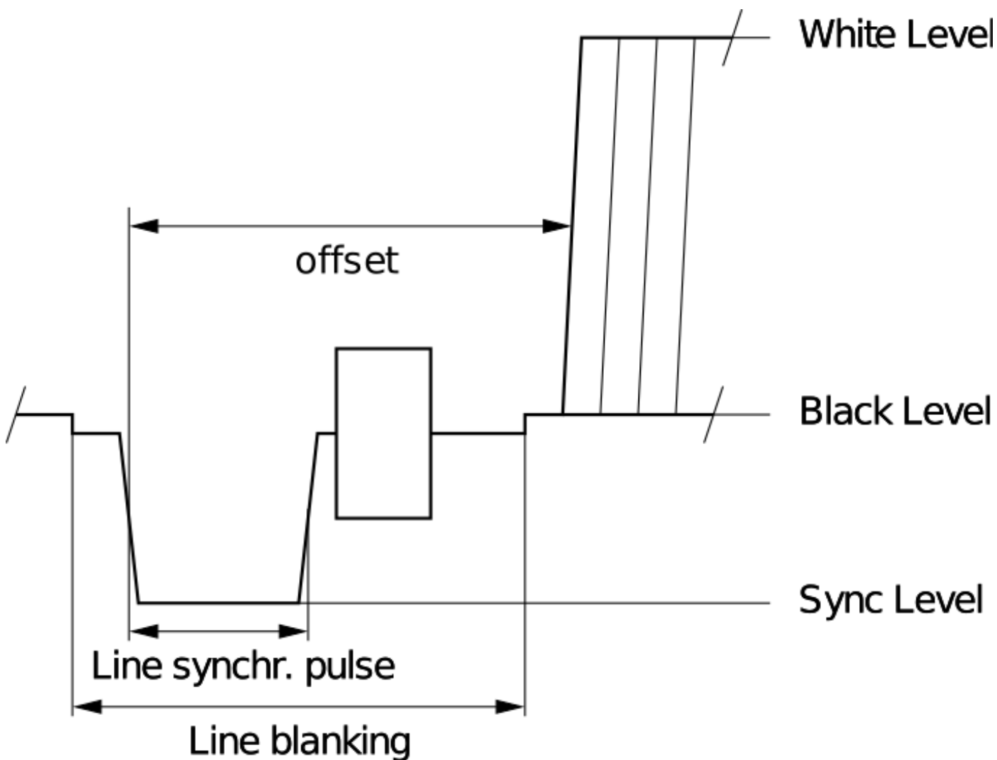
Fig. 1.8: Figure 4.1. Line synchronization
