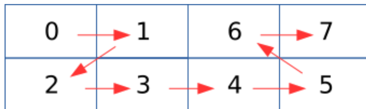
Fig. 1.4: V4L2_PIX_FMT_NV12MT macroblock Z shape memory layout
