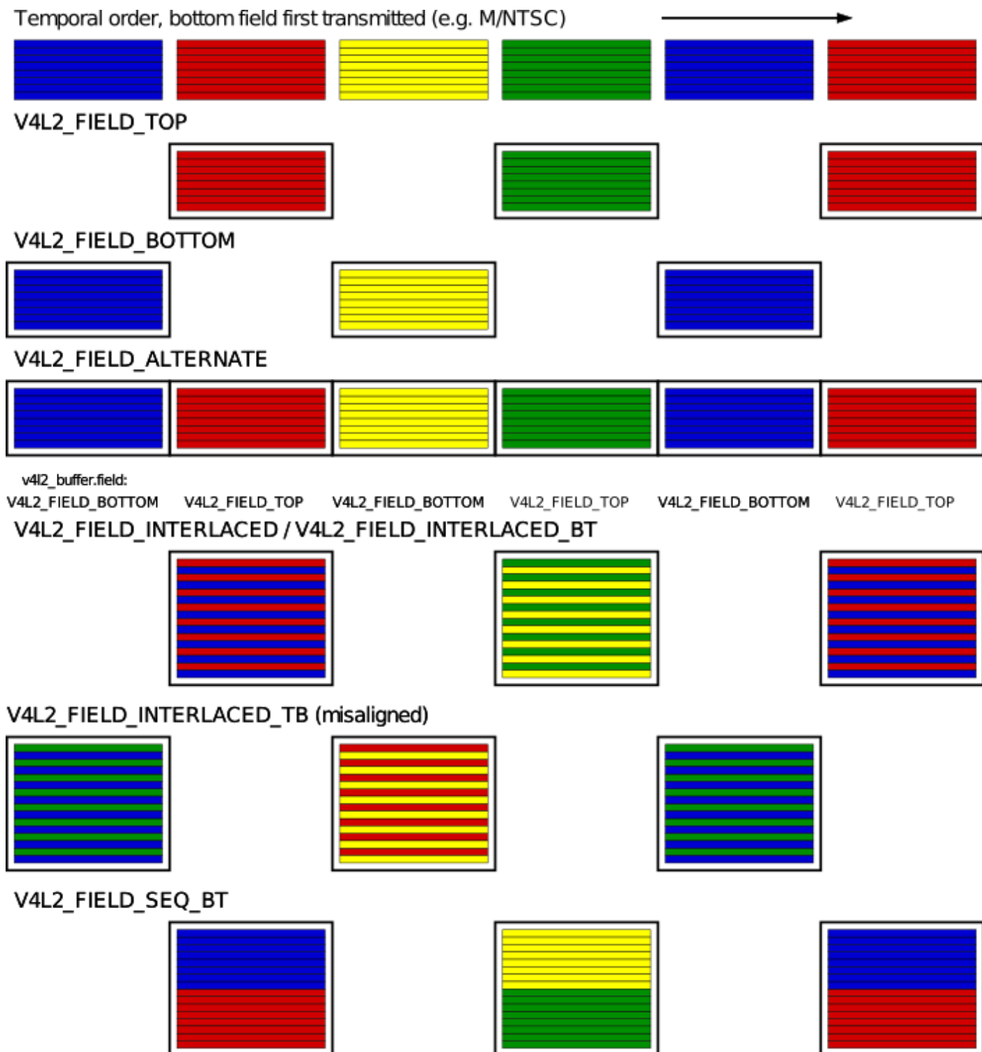
Fig. 1.7: Field Order, Bottom Field First Transmitted
