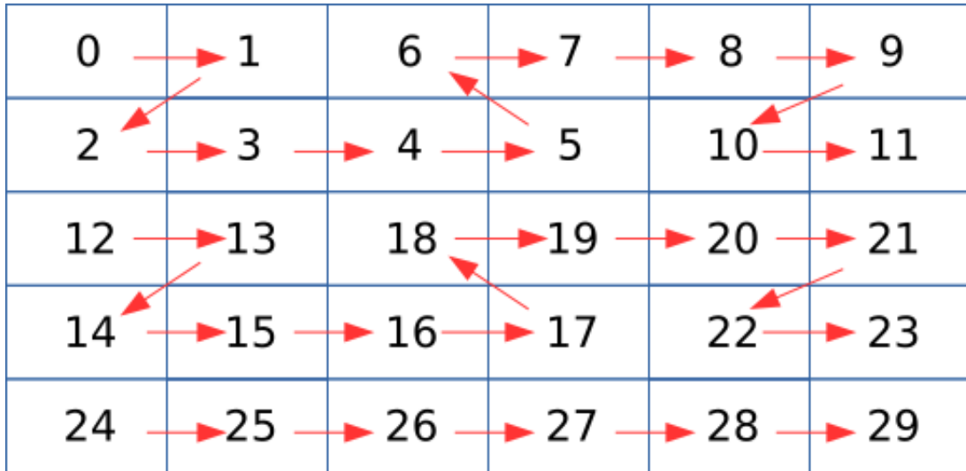
Fig. 1.5: Example V4L2_PIX_FMT_NV12MT memory layout of macroblocks
