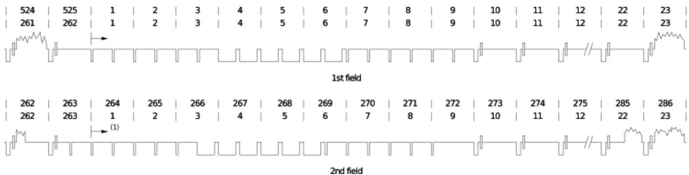
Fig. 1.9: Figure 4.2. ITU-R 525 line numbering (M/NTSC and M/PAL)
