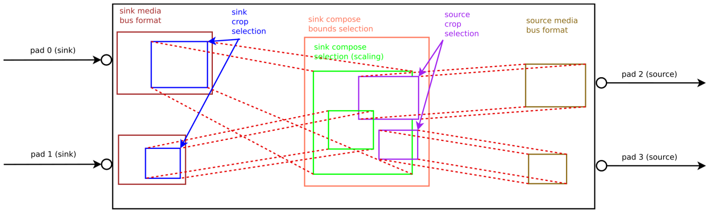
Fig. 1.14: Figure 4.7. Image processing in subdevs: scaling and composition with multiple sinks and sources
